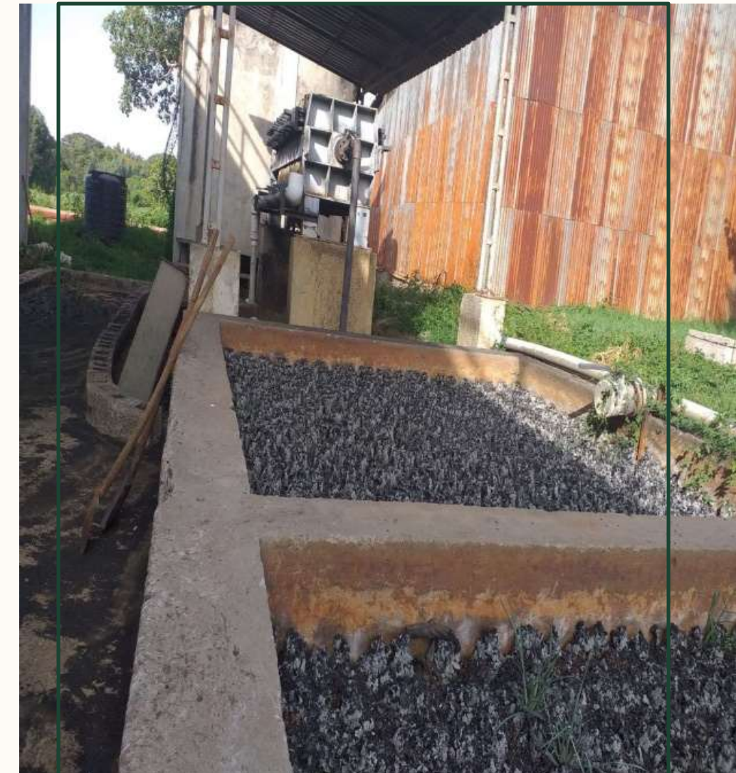
Sludge drying beds, Bahir Dar Textile Share Company
