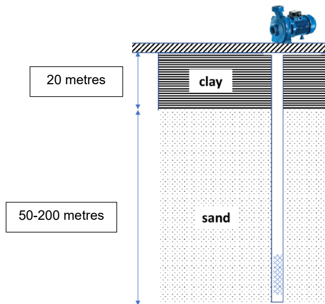
Figure 5: Soil profile in Hakimpur Upazila and location of tubewell screen.
