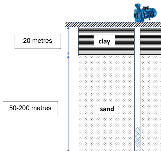
Figure 5: Soil profile in Satkania Upazila and location of tubewell screen.
