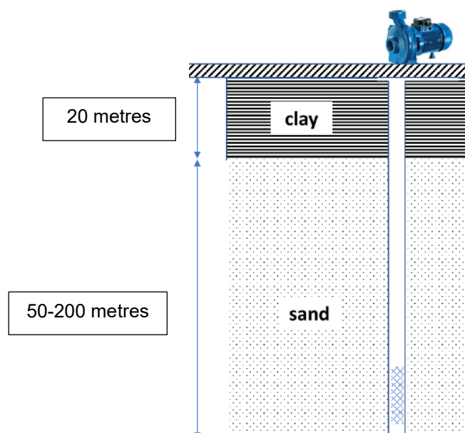
Figure 5: Soil profile in Banshkhali Upazila and location of tubewell screen.
