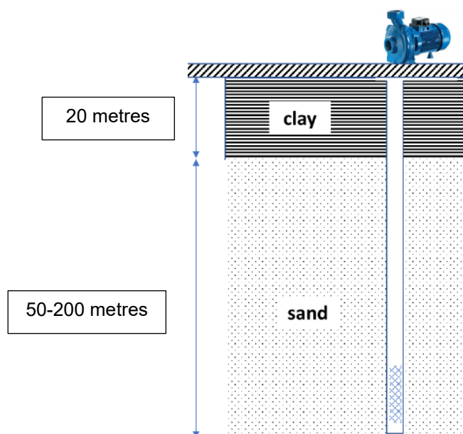
Figure 5: Soil profile in Sundarganj Upazila and location of tubewell screen.
