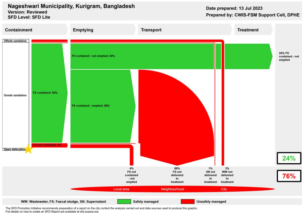
Figure 1: SFD Graphic for Nageshwari Municipality.
