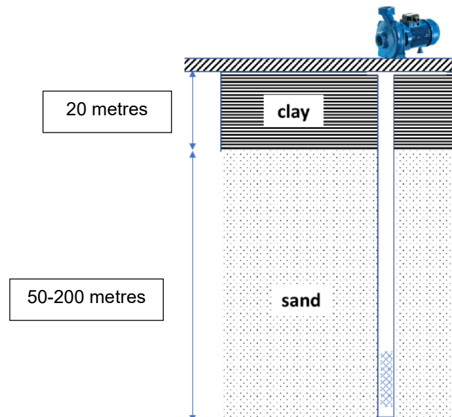
Figure 5: Soil profile in Nageshwari Upazila and location of tubewell screen.
