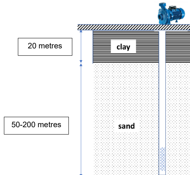
Figure 5: Soil profile in Patgram Upazila and location of tubewell screen.
