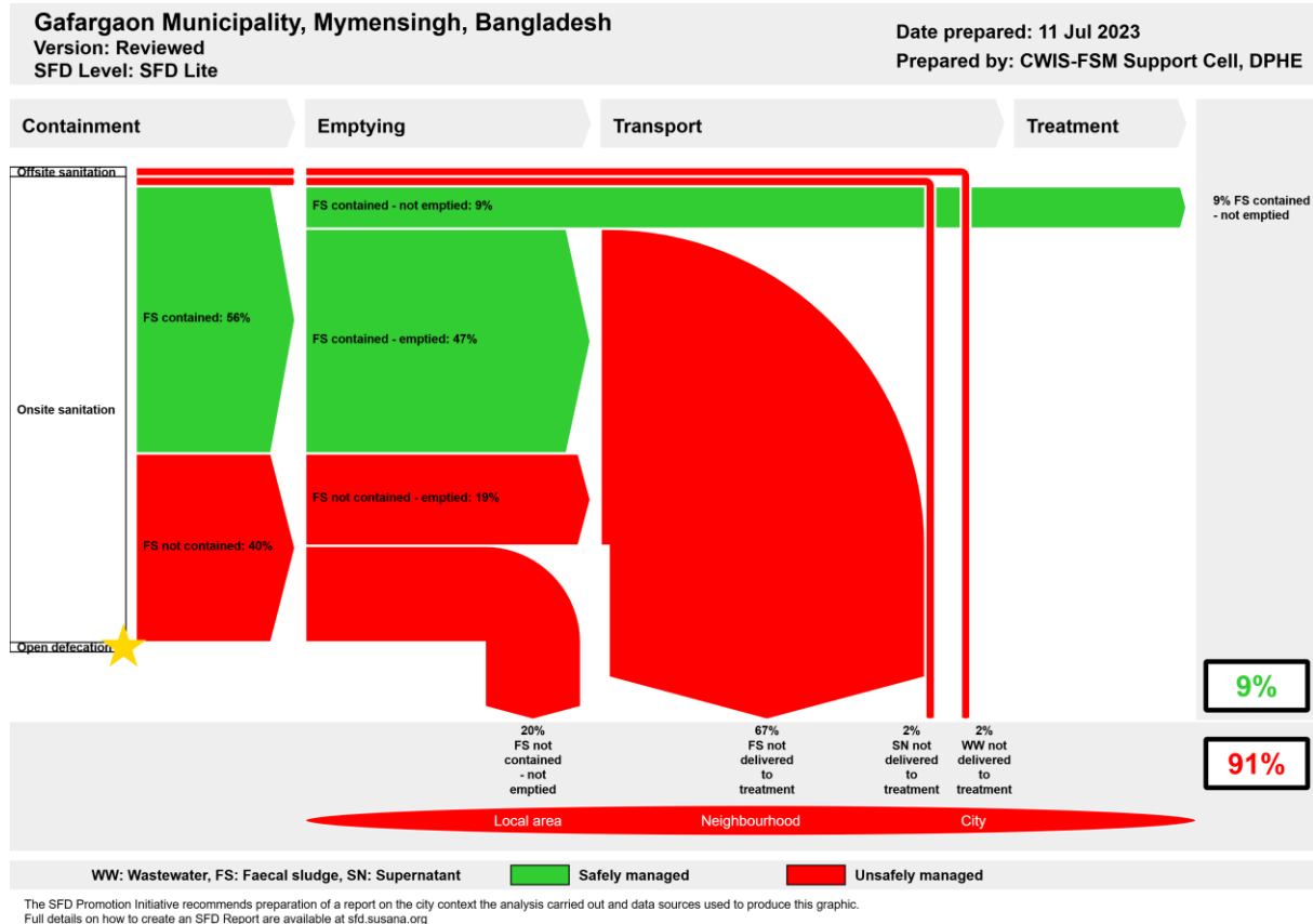
Figure 1: SFD Graphic for Gafargaon Municipality.
