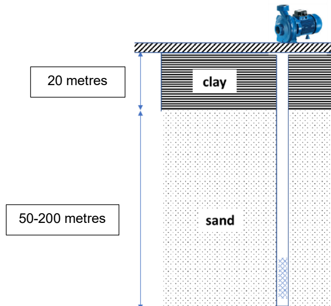
Figure 5: Soil profile in Gafargaon Upazila and location of tubewell screen.
