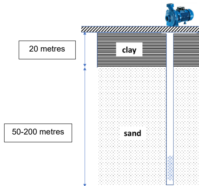
Figure 5: Soil profile in Shibchar Upazila and location of tubewell screen.
