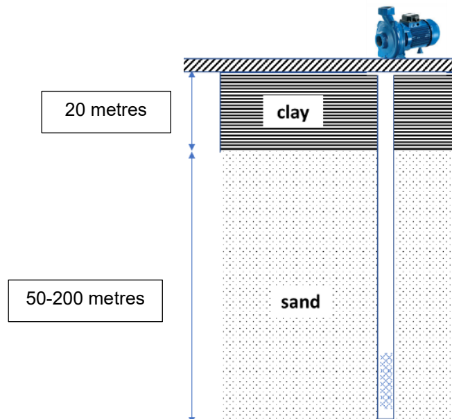
Figure 5: Soil profile in Chhatak Upazila and location of tubewell screen.
