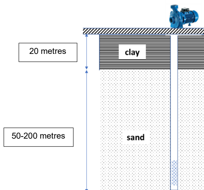
Figure 5: Soil profile in Islampur Upazila and location of tubewell screen.
