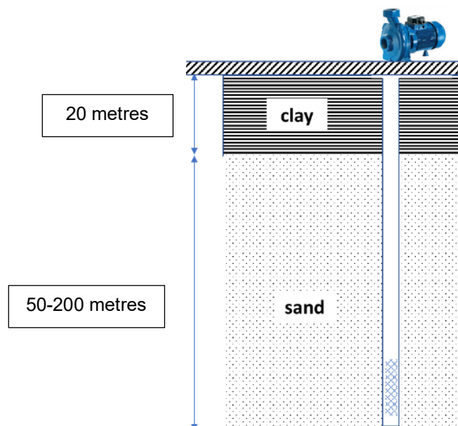
Figure 5: Soil profile in Pirojpur district and location of tubewell screen.
