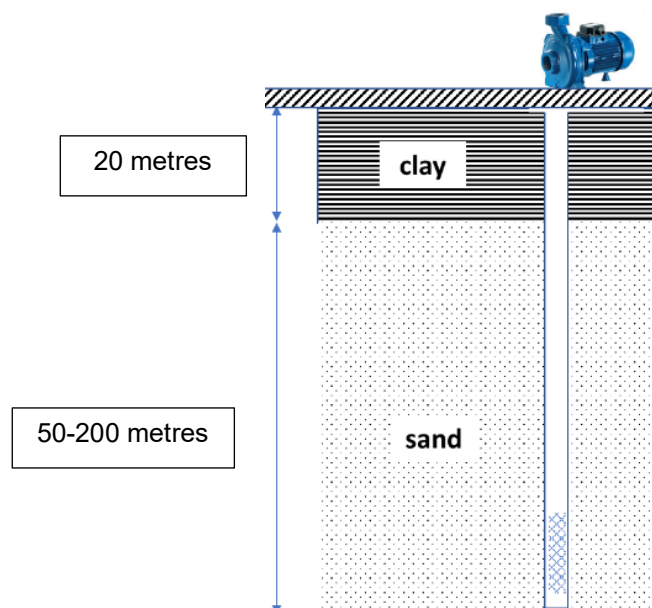
Figure 5: Soil profile in Netrokonadistrict and location of tubewell screen.
