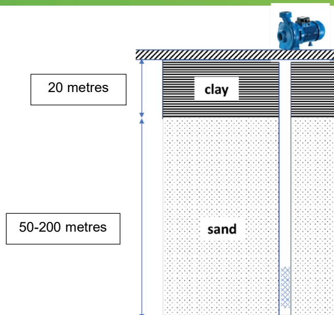
Figure 5: Soil profile in Satkhira district and location of tubewell screen.
