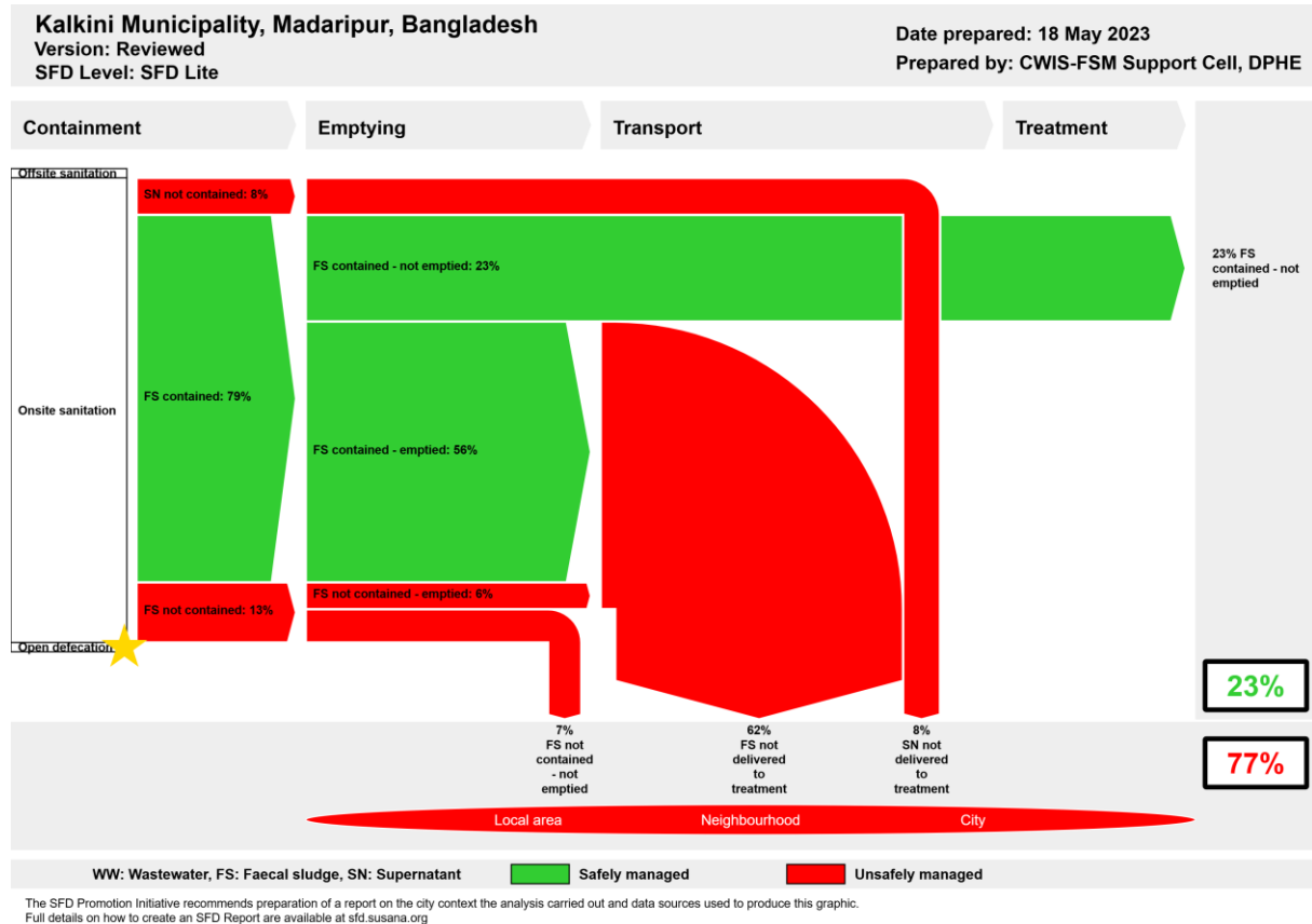
Figure 7: SFD Graphic for Kalkini Municipality.
