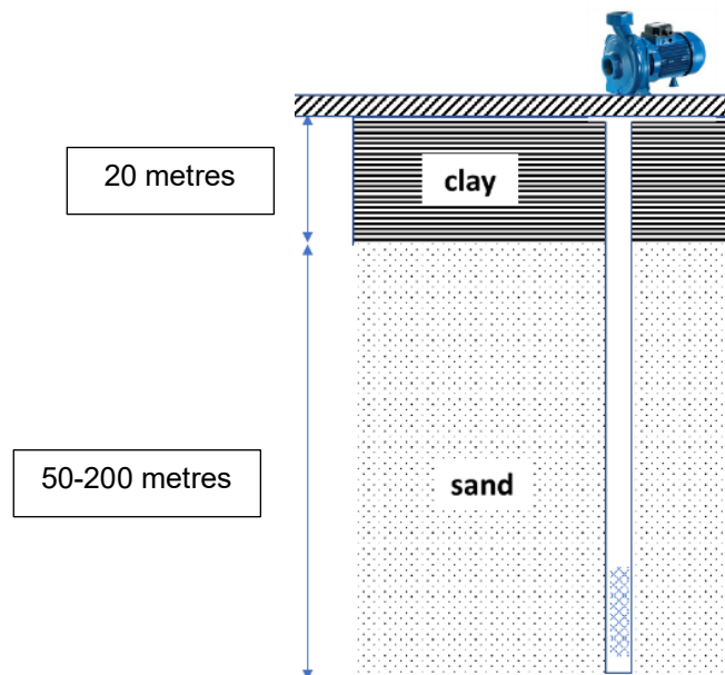
Figure 5: Soil profile in Kalkini Upazila and location of tubewell screen.
