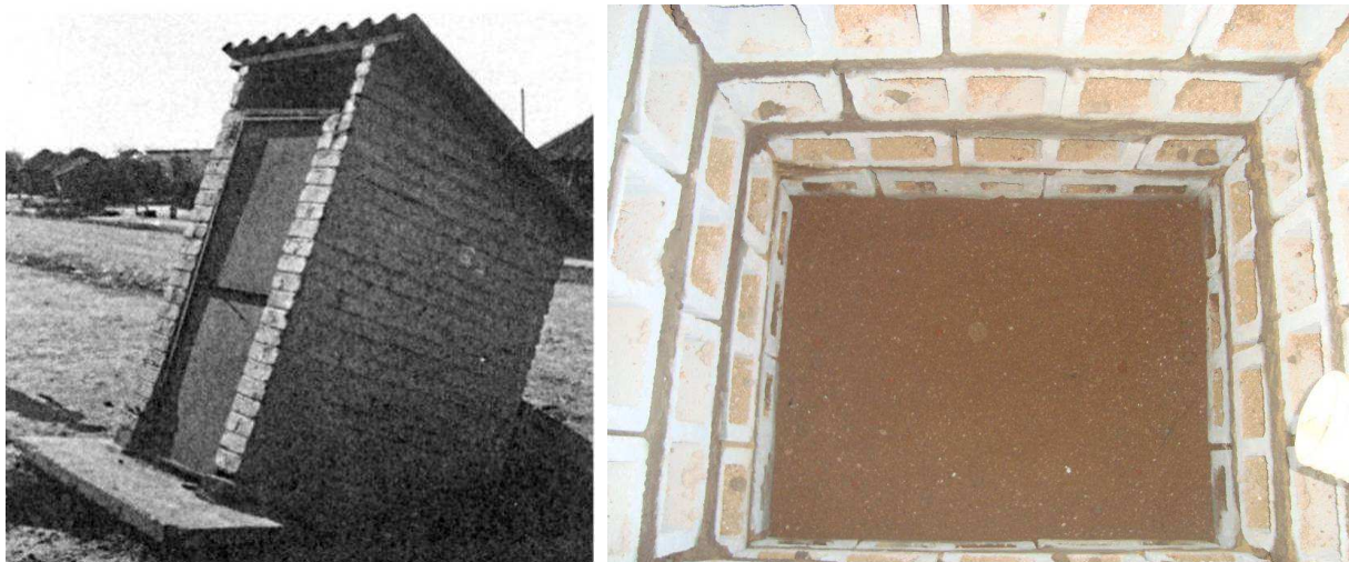
Figure 2.1 Left: An unlined or unreinforced pit cannot support a heavy top structure. Right: A pit lined with blocks laid with open vertical joints, allowing drainage through the bottom and sides of the pit.
